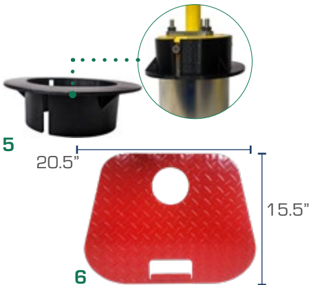
5. Hole Cutter Flanged Stop [No. 217PL] Adjustable flanged stop ensures proper hole depth every time.
