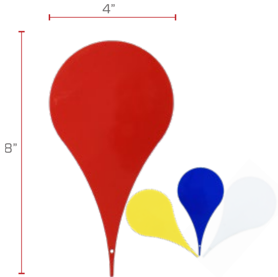
● Red ○ White ● Blue ● Yellow Made of 1/8" thick steel with powder coated finish. Custom decals and colors are available. Tear Drop Tee Marker [No. 816] Raw/Unfinished Markers are available. *Custom decal available* - Call for quote.
